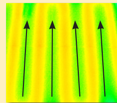
Infrared image using standard tile adhesive shows cold spots between wires
