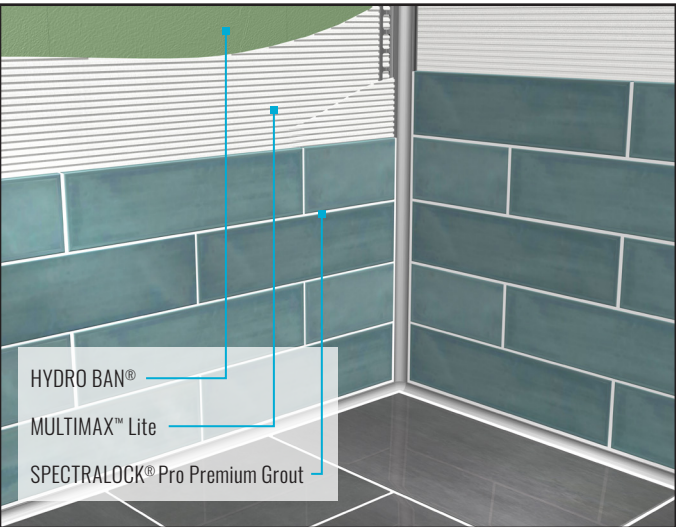
COVE PROFILE
