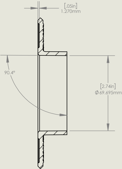
SECTION B-B
