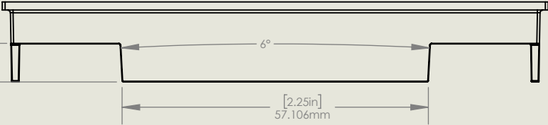
SECTION F-F
