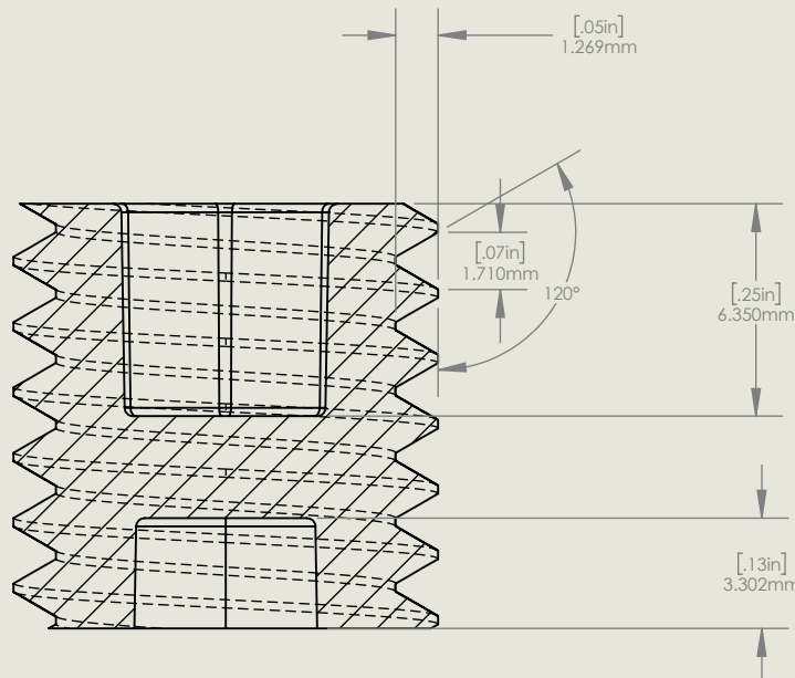
SECTION H-H
