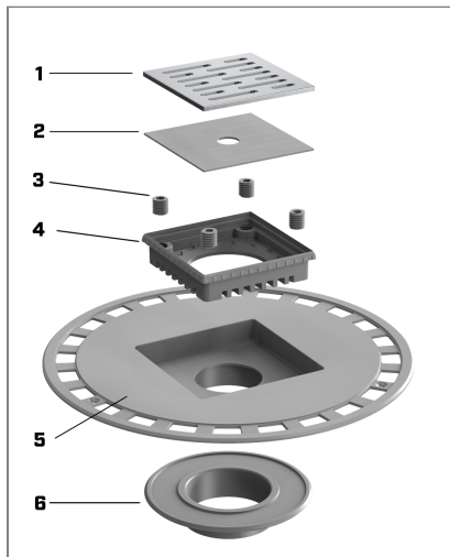
4 x 4 Metal Grate Assembly (FIG 1)
