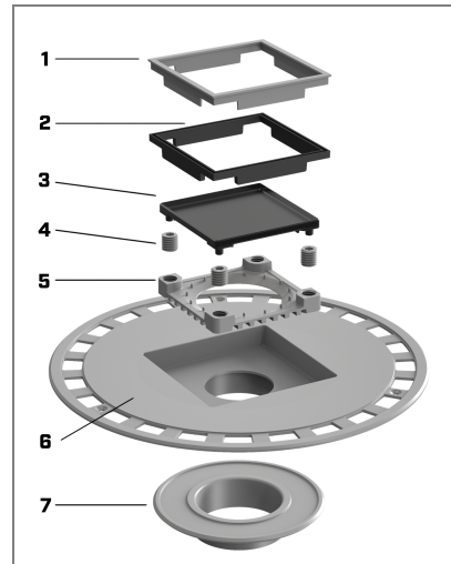
4 x 4 Tile-in Assembly (FIG 2)
